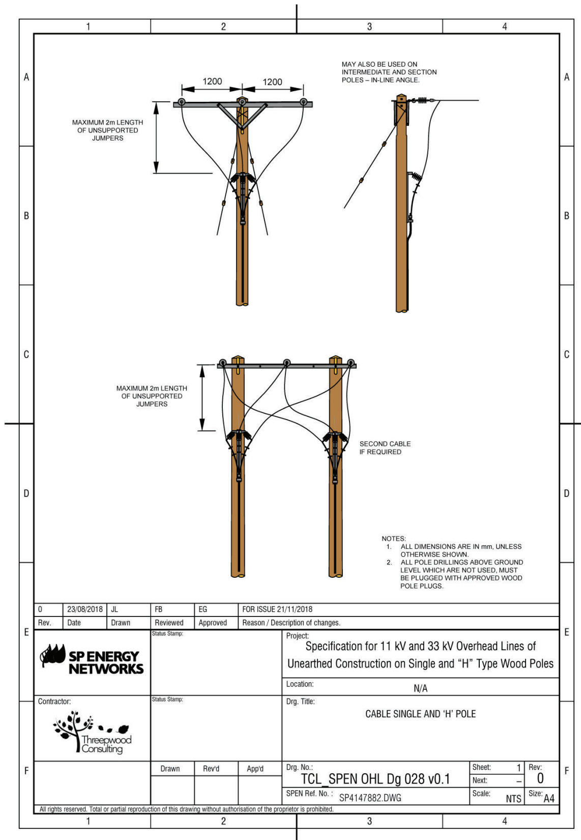
22.28 Figure 28 General Arrangement Cable Single and "H" Pole (Drawing No. SP4147882)
